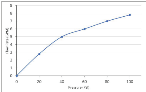
V-2307B Flow Rate (GPM) Vs Pressure (PSI) For Tub Port*
